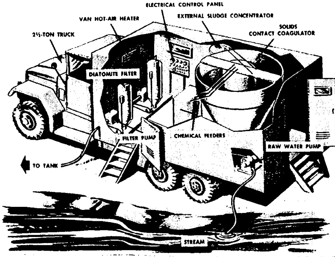
Figure 5-3. Water purification unit, van type body mounted. This entire device is commonly known as an erdlator
